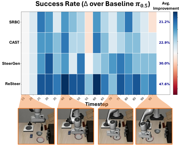
Fig. 7. We conduct a case study on task steering from Push the Plate to the Front of the Stove \rightarrow Put the Bowl on the Plate . The prompt is switched at the indicated timestep, with representative LIBERO environment states shown at select timesteps. SteerGen and ReSteer consistently outperform all baseline methods, with particularly strong gains at later timestep switches. ReSteer further improves upon SteerGen by sharpening the policy in regions where SteerGen cannot consistently complete the task.
