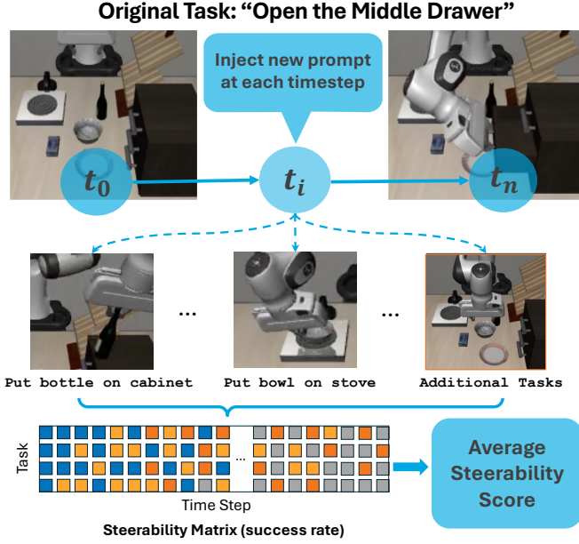
Fig. 2. Steerability evaluation. We run an original task i , then at sampled timesteps t we switch the language prompt to a target task j and measure whether the policy completes j from that state. Repeating this over all sampled states and all target tasks yields a steerability matrix (time \times target task), whose average success rate gives the overall steerability score in task i .
